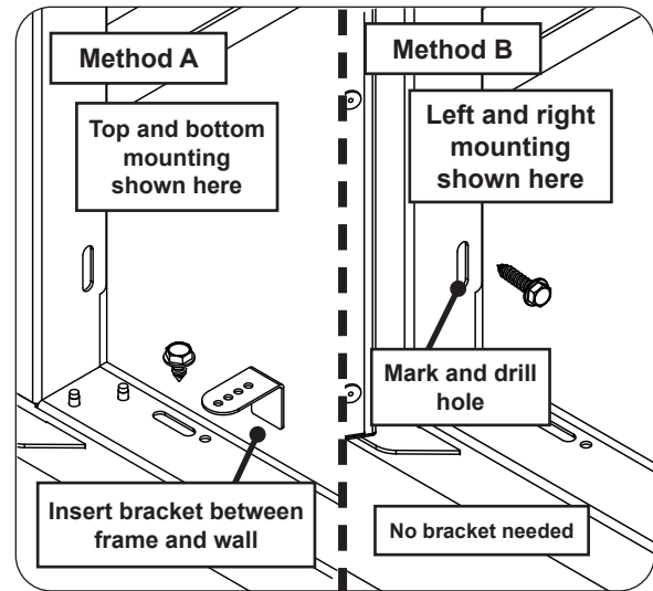
Fig. 2-3 Installation methods
