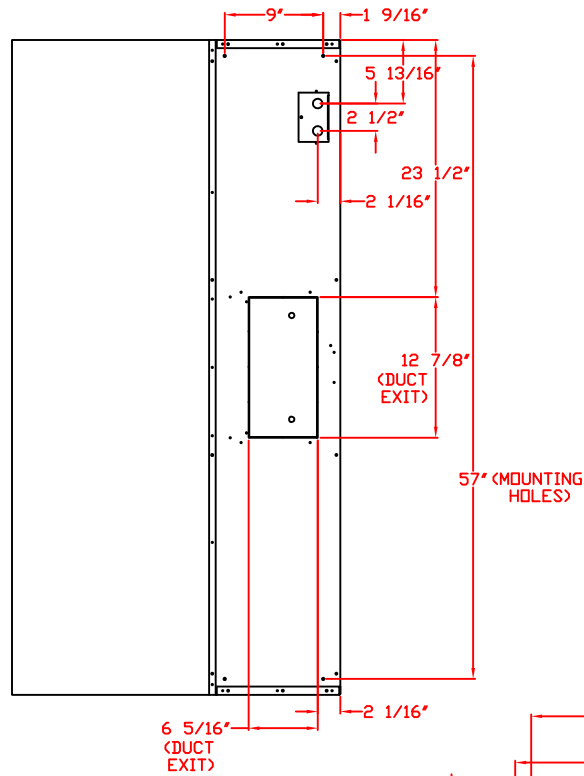
TOP VIEW (DUCT EXIT SHOWN IN TOP LOCATION)
